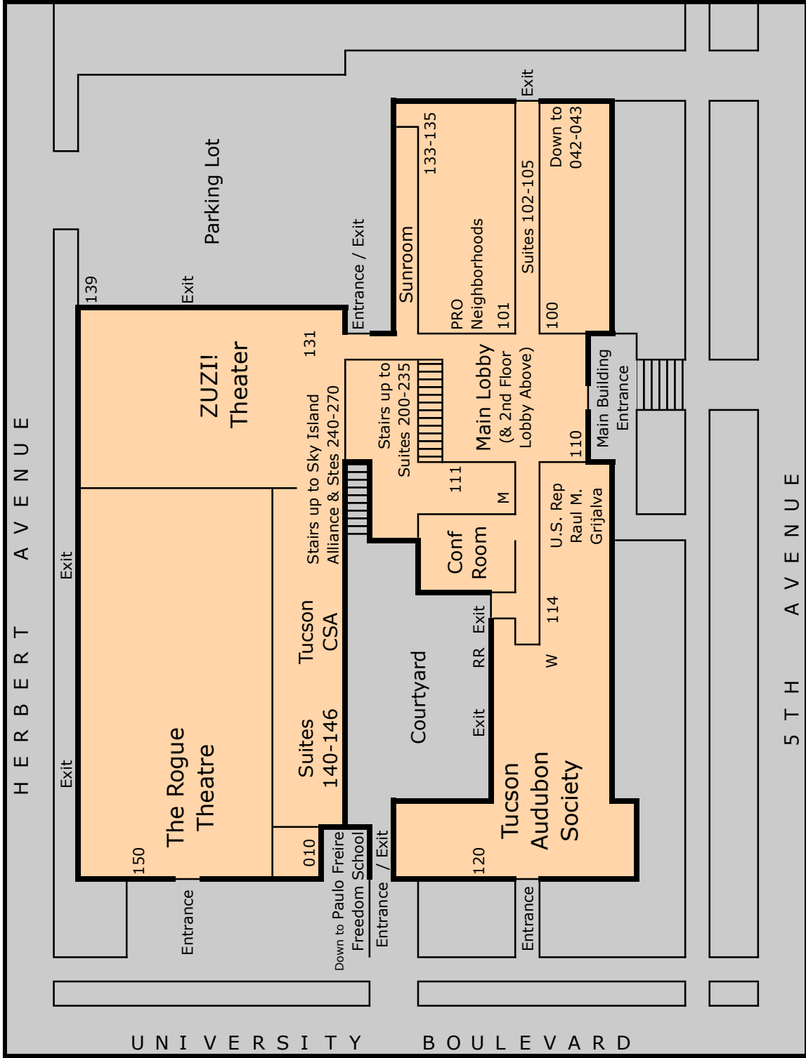
THE HISTORIC Y - FIRST FLOOR PLAN - NOV 2011
